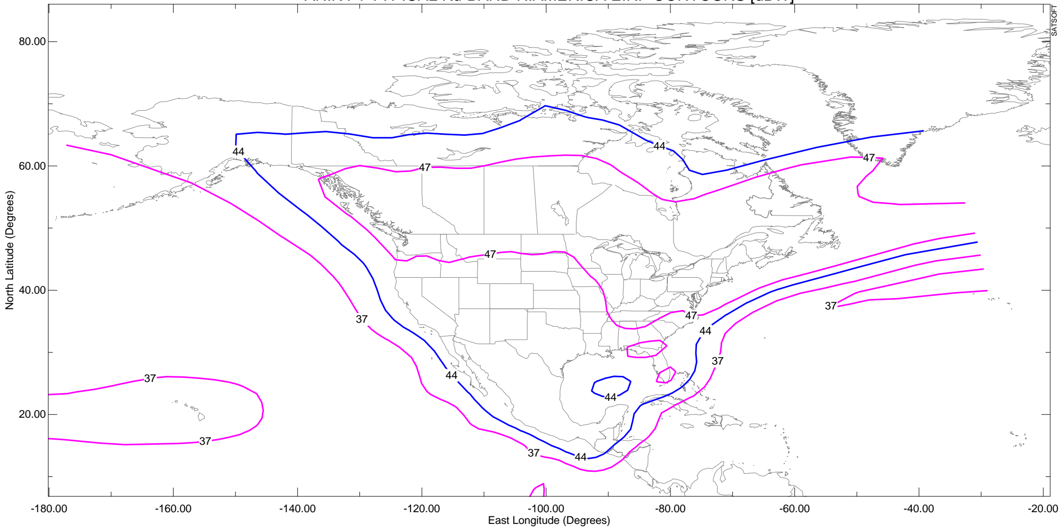
ANIK F1 TYPICAL Ku-BAND N.AMERICA EIRP CONTOURS [dBW]
